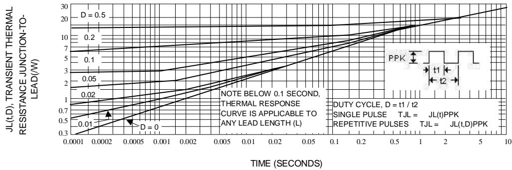
Fig. 3-TYPICAL THERMAL RESPONSE
