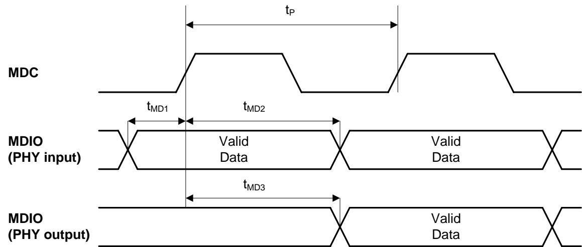
Figure 19. MDC/MDIO Timing
