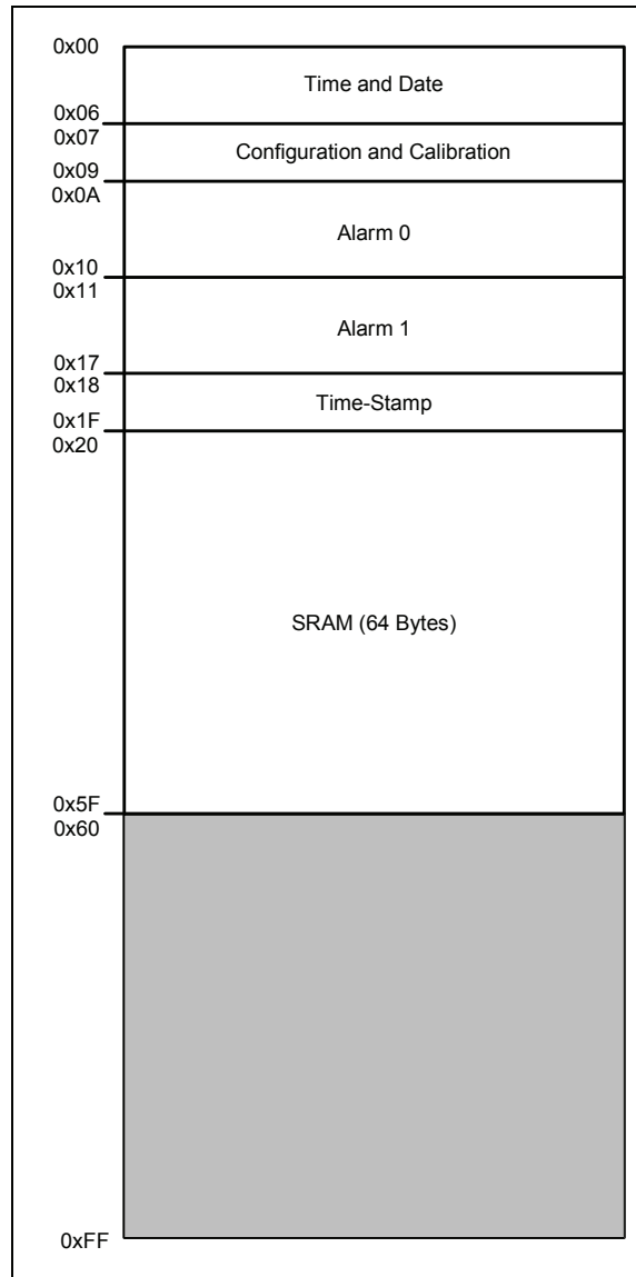
FIGURE 4-1: MEMORY MAP
