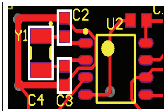
FIGURE 4-3: BOARD LAYOUT
