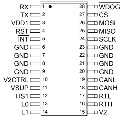
Figure 2. 33889 Pin Connections
