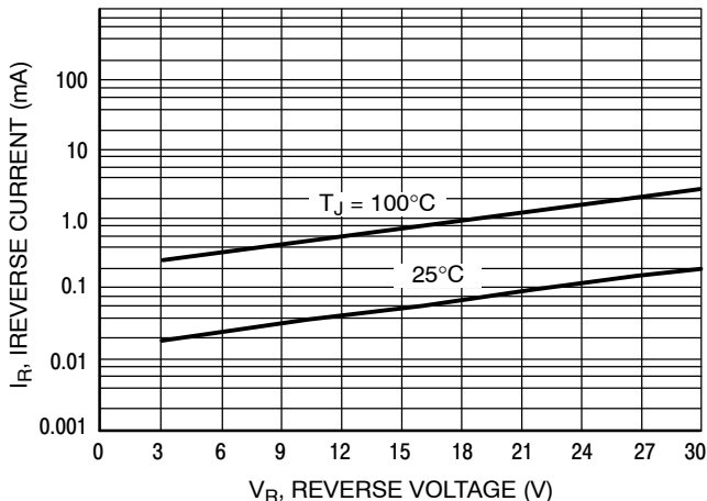
Figure 3. Typical Reverse Leakage Current
