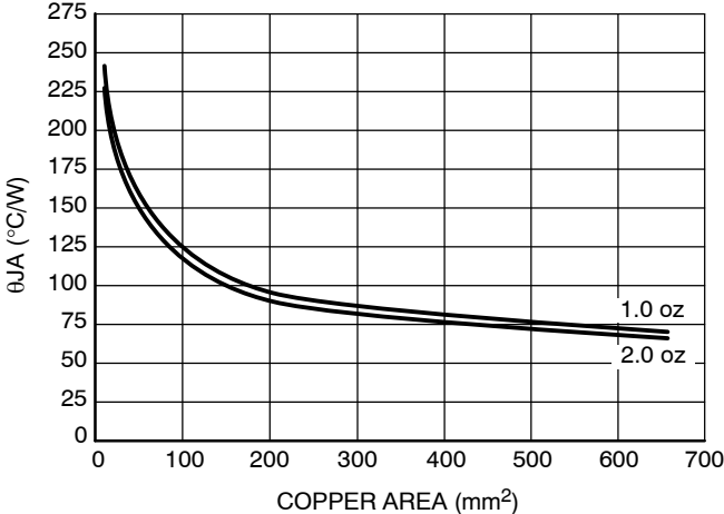
Figure 10. Thermal Resistance vs. Copper Area
