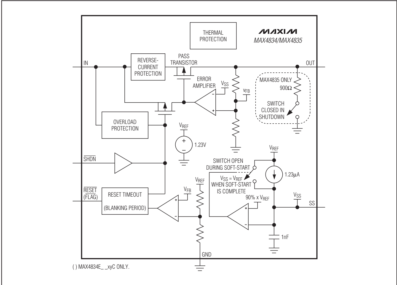
Figure 1. Functional Diagram
