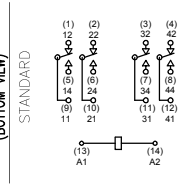
CONNECTION DIAGRAM (BOTTOM VIEW)
