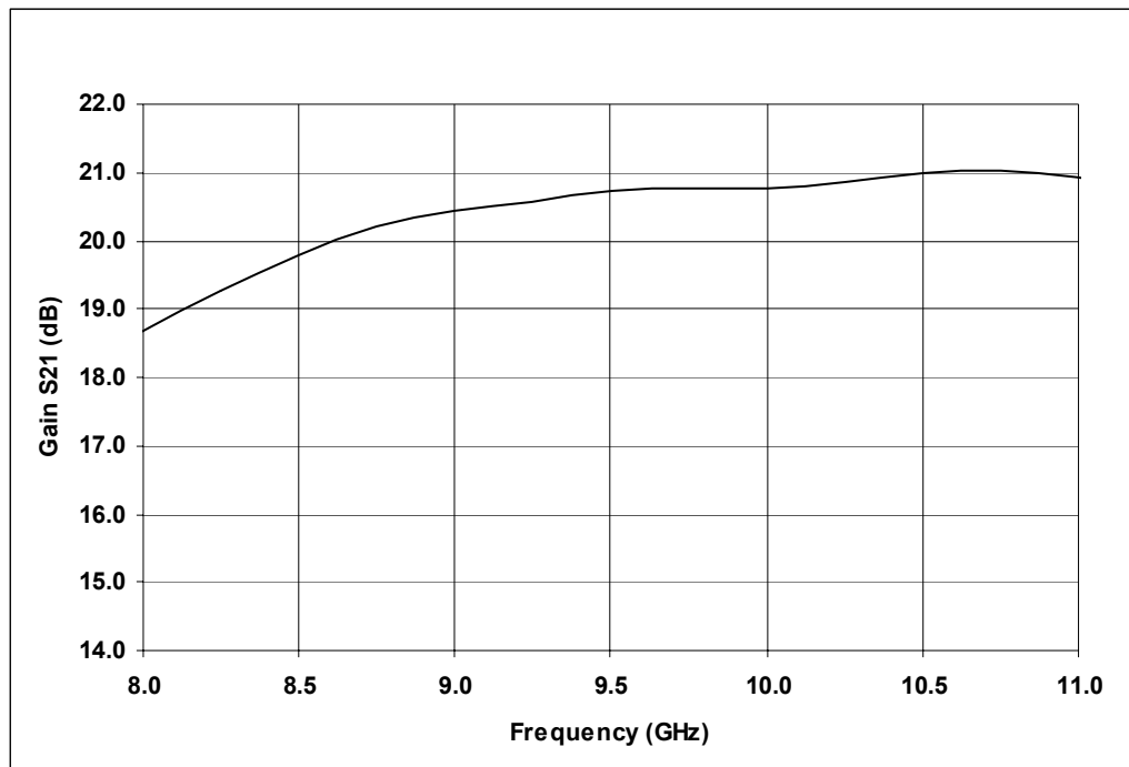
Figure 1. Gain
