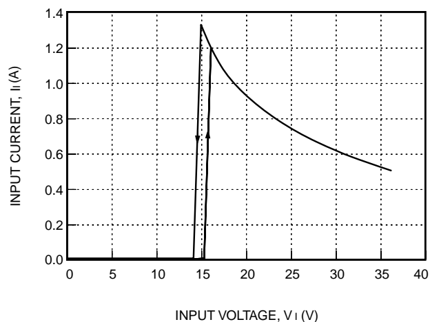
Figure 2. LC015 Input Current vs. Input Voltage at I_o = I_{o, max} and T_c = 25^\circ C
