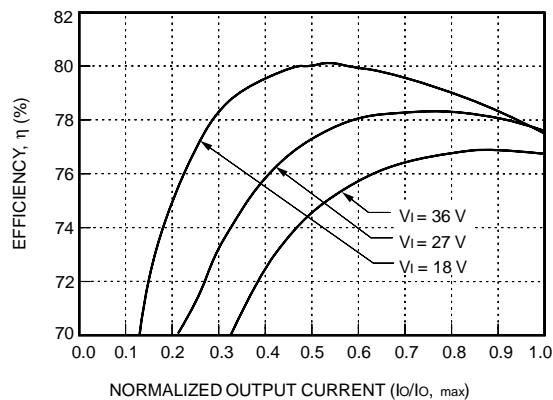
Figure 19. LC010A, B, C Typical Efficiency vs. Normalized Output Current at T_c = 25\text{ }^\circ\text{C}
