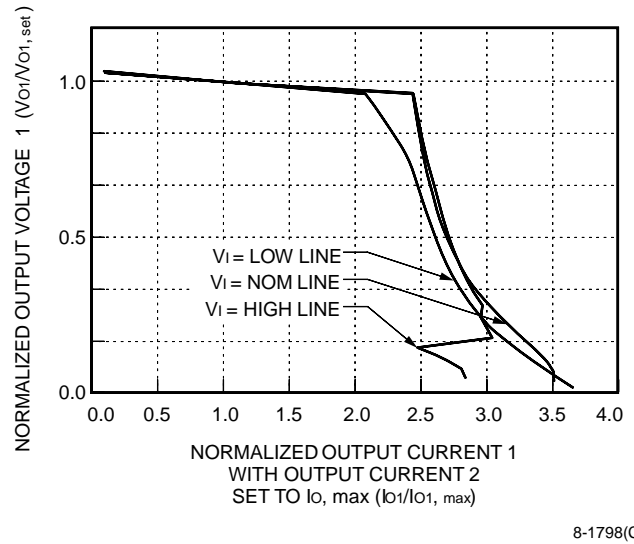
Note: Output2 has characteristics similar to output1 when output1 is set to I_{o, \max} .
