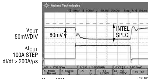
Load Transient with AVP
