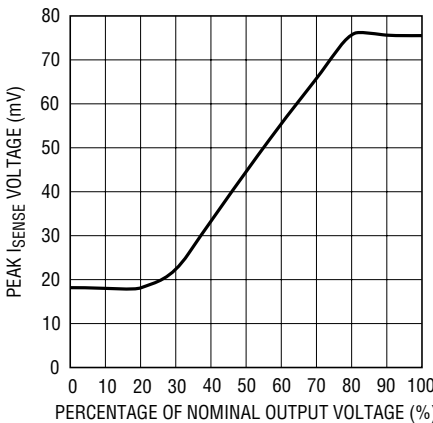
Percentage of Nominal Output vs Peak I_{\text{SENSE}} (Foldback)
