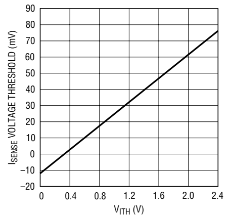
Peak Current Threshold vs V_{I\text{TH}}
