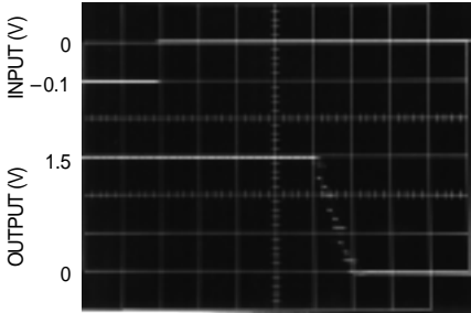
Input Overload Recovery
