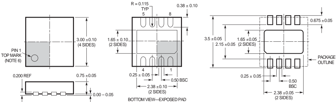
RECOMMENDED SOLDER PAD PITCH AND DIMENSIONS (03) DFN 1003
