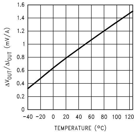
DC Load Regulation
