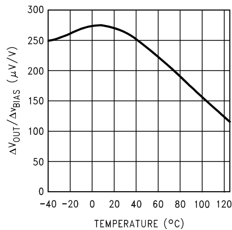
Line Regulation vs V_{BIAS}
