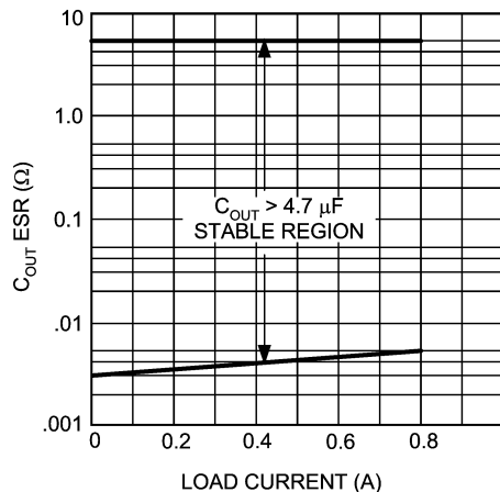
Minimum ESR vs Output Load Current 20063031
