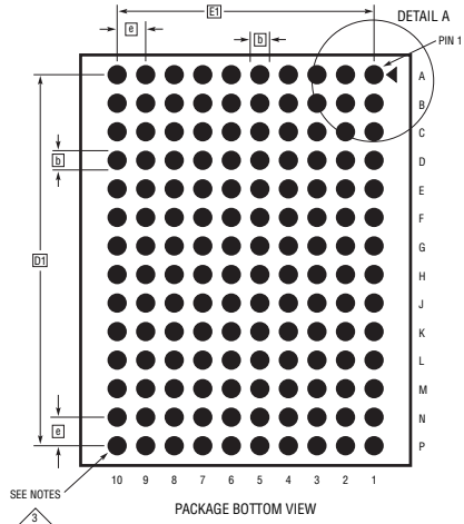
PACKAGE BOTTOM VIEW
