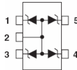
SC-88A/SOT-323
