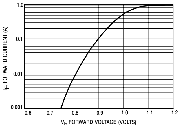
Figure 5. Forward Voltage
