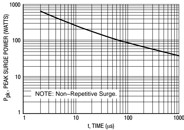
Figure 1. Pulse Width
