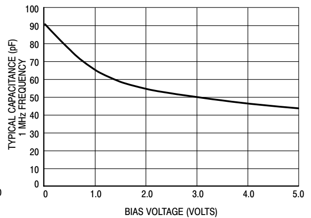
Figure 4. Capacitance
