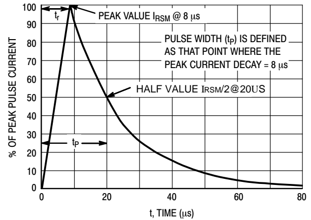
Figure 2. 8 x 20 µs Pulse Waveform
