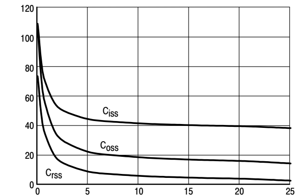
Figure 11. Capacitance
