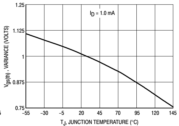
Figure 4. Threshold Voltage Variation with Temperature
