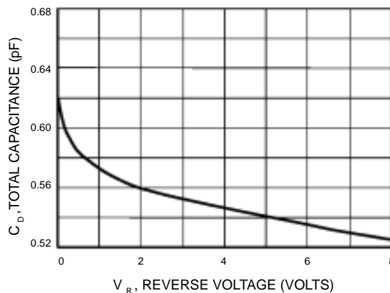
Figure 4. Capacitance
