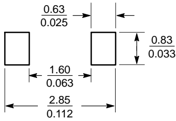
SOLDERING FOOTPRINT*
