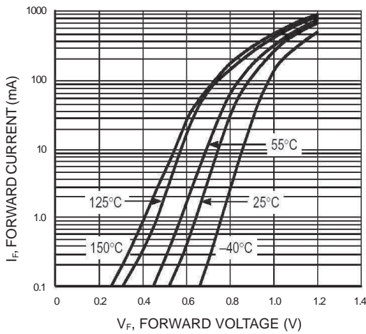
Figure 2. Forward Current
