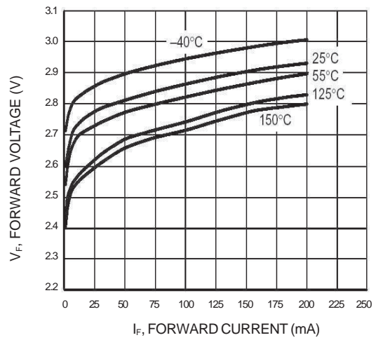
Figure 5. Forward Voltage
