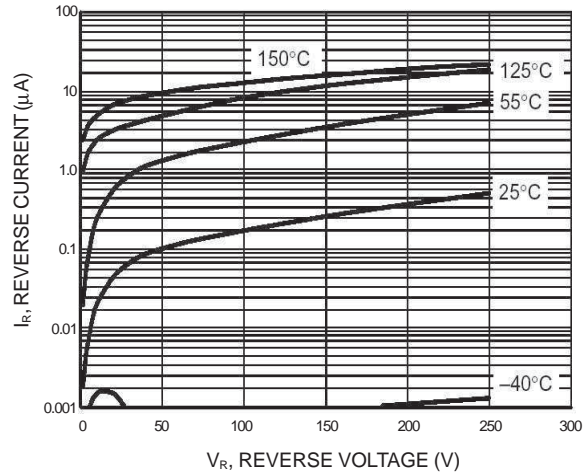
Figure 3. Leakage Current
