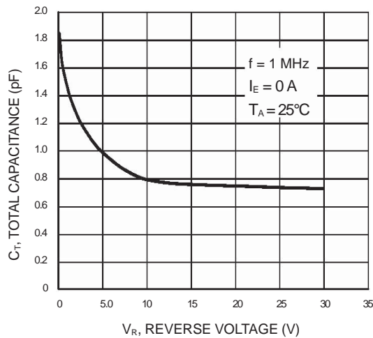
Figure 4. Total Capacitance
