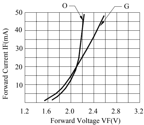
Fig.3 FORWARD CURRENT VS. FORWARD VOLTAGE PER CHIP
