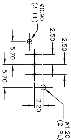
RECOMMENDED P.C.B. LAYOUT SCALE 2:1
