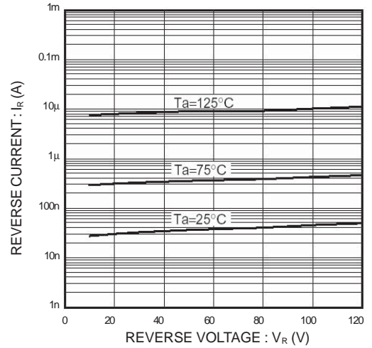
Fig.2 Reverse characteristics
