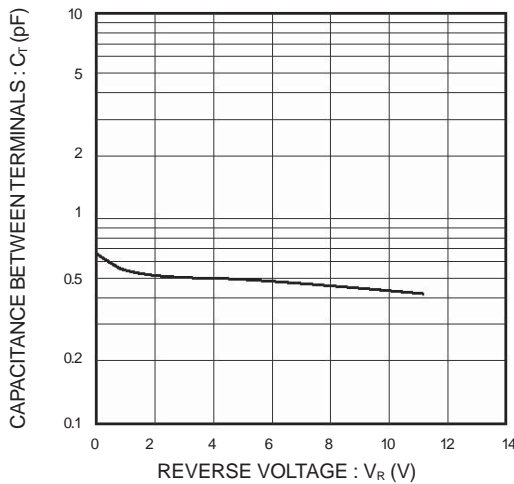
Fig.3 Capacitance between terminals
