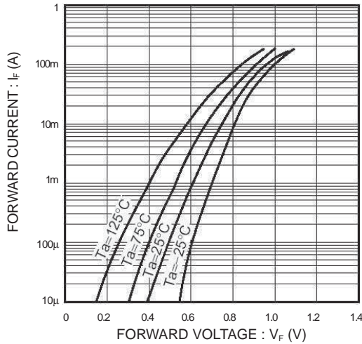
Fig.1 Forward characteristics
