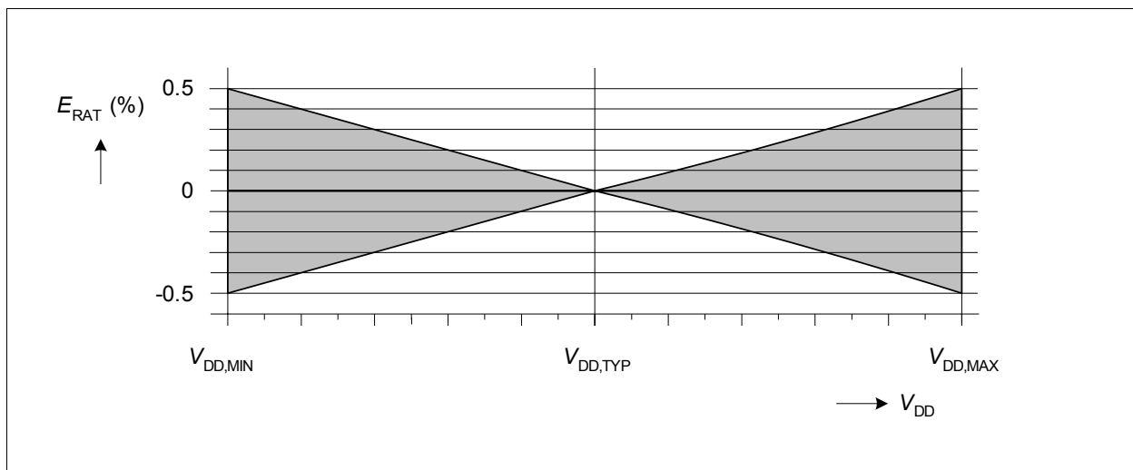
Figure 8 Ratiometric Error
