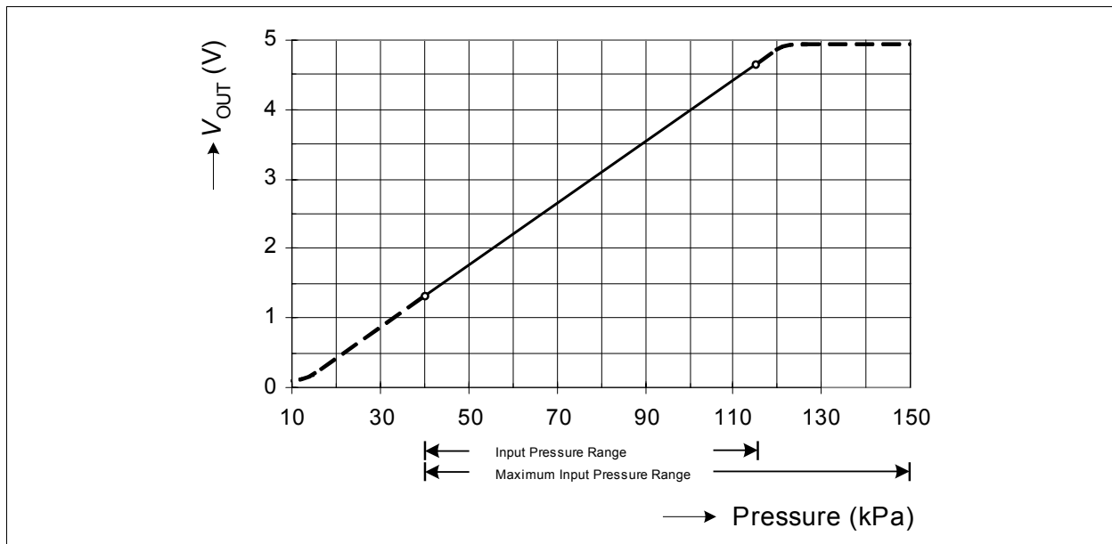
Figure 3 Transfer Function
