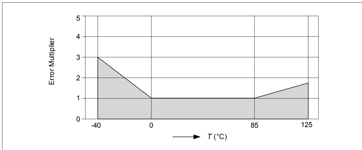
Figure 9 Error Multiplier over Temperature
