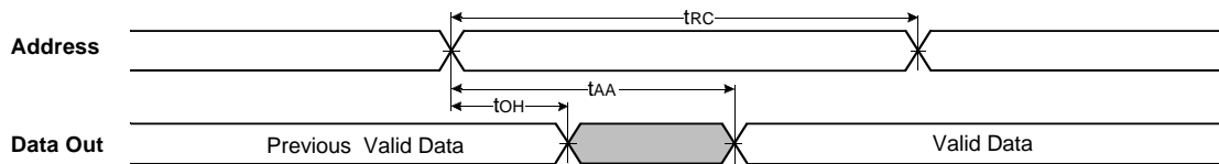
TIMING WAVEFORM OF READ CYCLE(1) ( \overline{CS}=\overline{OE}=V_{IL} , \overline{WE}=V_{IH} )
