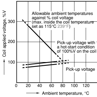
5.-(4) Ambient temperature characteristics (High sensitivity type) Contact current: 10 A
