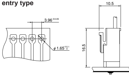
Locking header Top entry type
