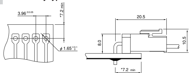
Locking header Side entry type
