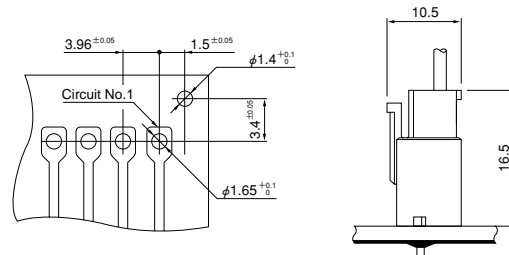
Shrouded header
