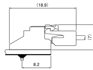
PAF Receptacle + PA side entry type header
