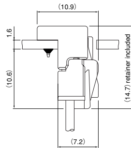
PA Receptacle (Retainer mountable type) + PA bottom type header
