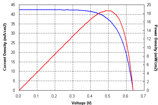
Current-Voltage Characteristics
