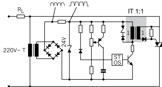
Triac phase angle control
