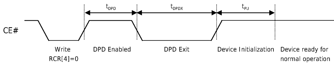
Figure 18: DPD Entry and Exit Timing Parameters
