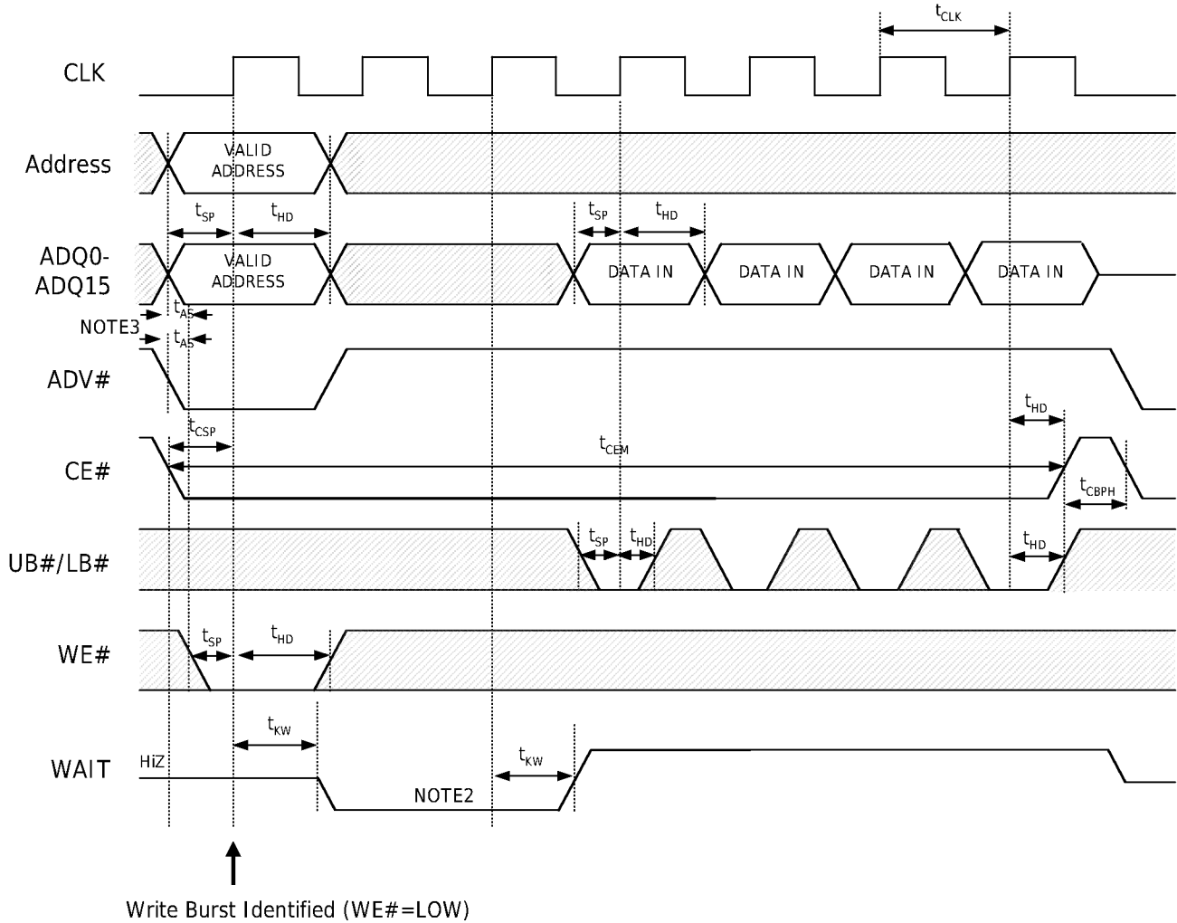
Figure 29: Four-Word Burst WRITE Operation - Variable Latency
