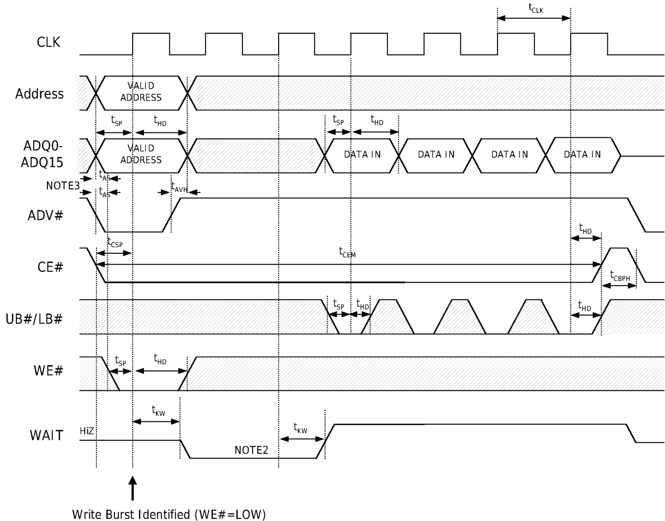
Figure 30: Four-Word Burst WRITE Operation - Fixed Latency
