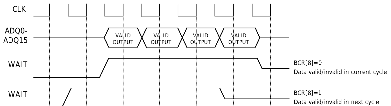
Figure 12. WAIT Configuration During Burst Operation
