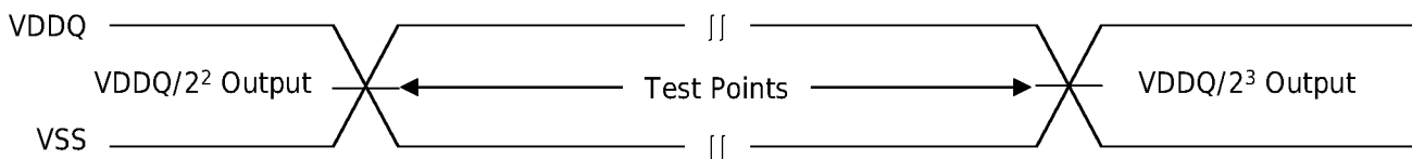
Figure 15. AC Input/ Output Reference Waveform
