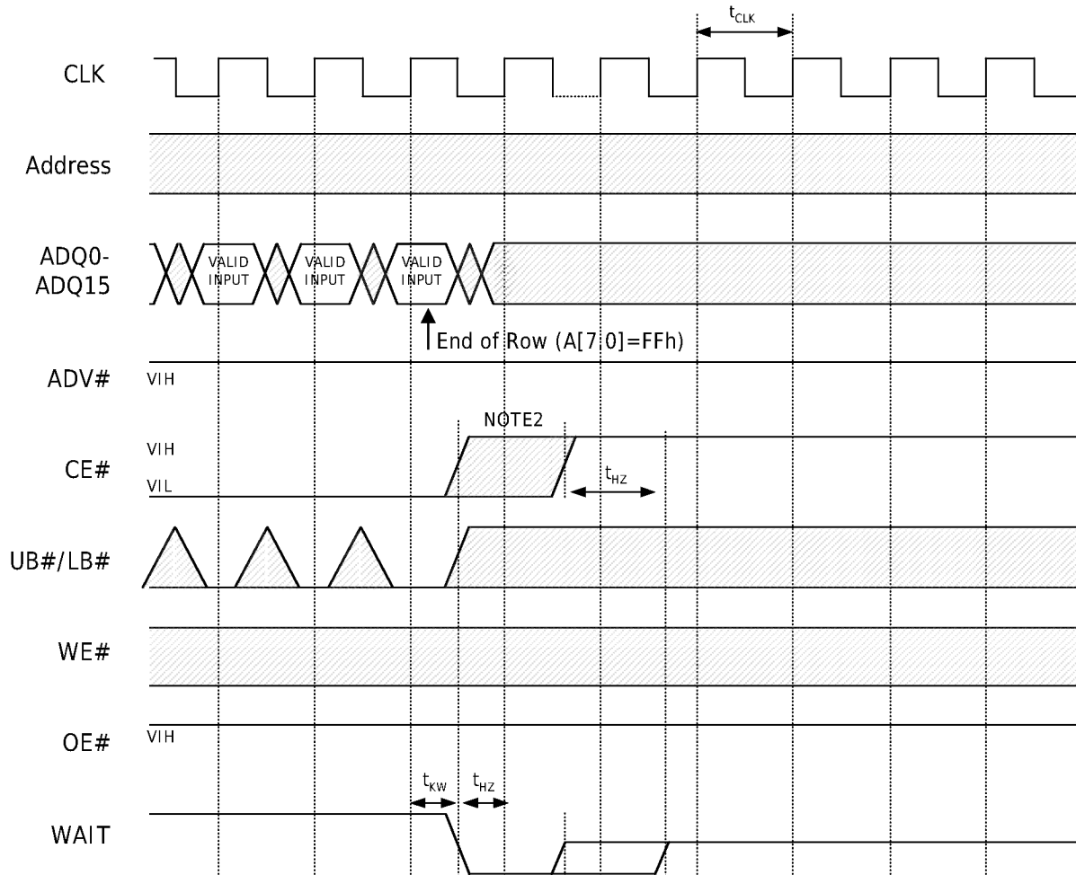
Figure 31: Continuous Burst WRITE at End-of-Row (Wrap Off)
