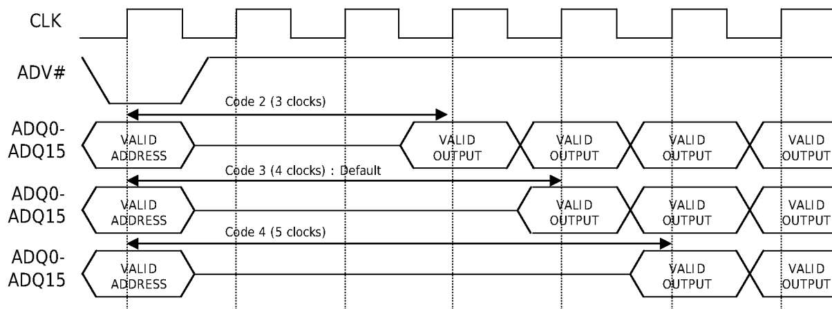
Figure 13. Latency Counter (Variable Latency, No Refresh Collision)
