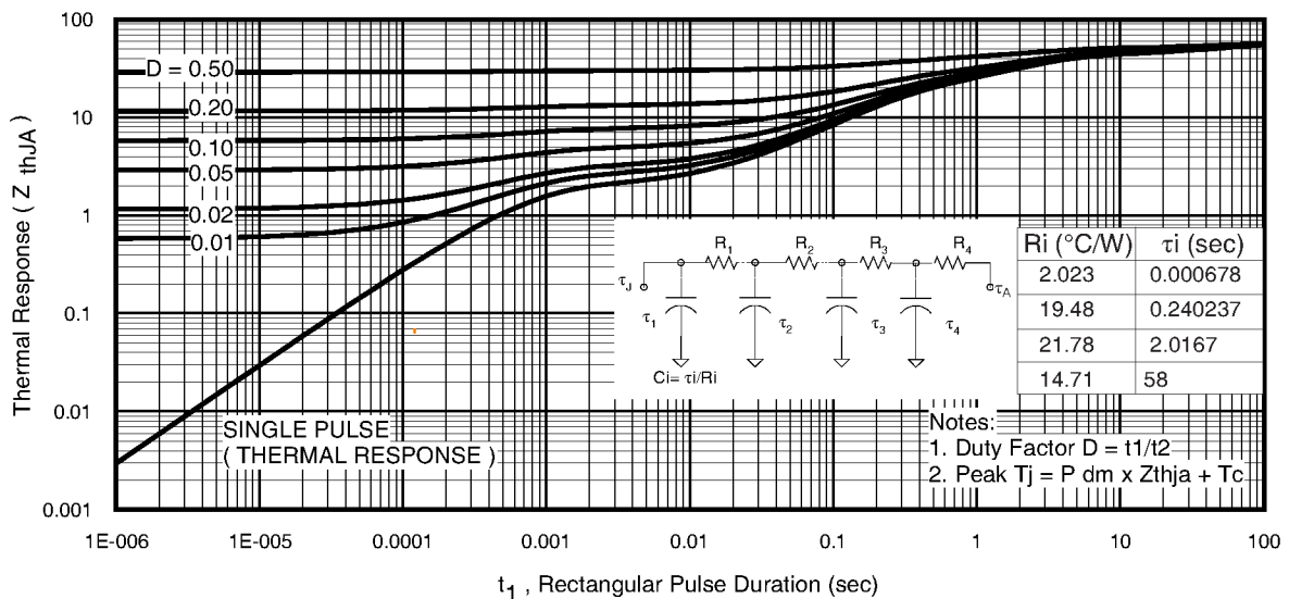
Fig 11. Maximum Effective Transient Thermal Impedance, Junction-to-Air
