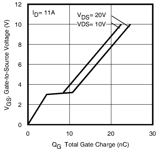
Fig 6. Typical Gate Charge Characteristics www.irf.com
