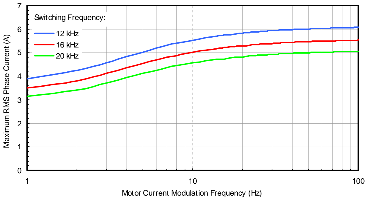
Figure 4. Maximum sinusoidal phase current as function of modulation frequency V_{BUS}=400\text{V} , T_j=150^\circ\text{C} , T_c=100^\circ\text{C} , Modulation Depth=0.8, PF=0.6
