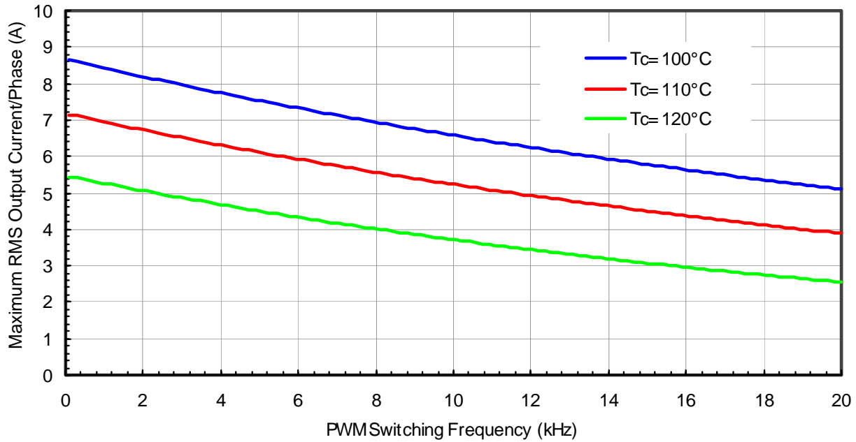
Figure 3. Maximum sinusoidal phase current as function of switching frequency V_{BUS}=400\text{V} , T_j=150^\circ\text{C} , Modulation Depth=0.8, PF=0.6
