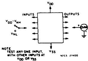
Fig. 10 - Noise immunity test circuit.
