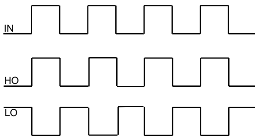
Figure 1. Input/Output Timing Diagram
