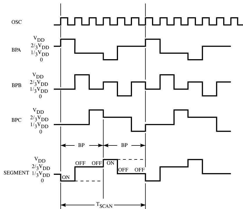
Figure 2. Backplane and Segment Waveforms
