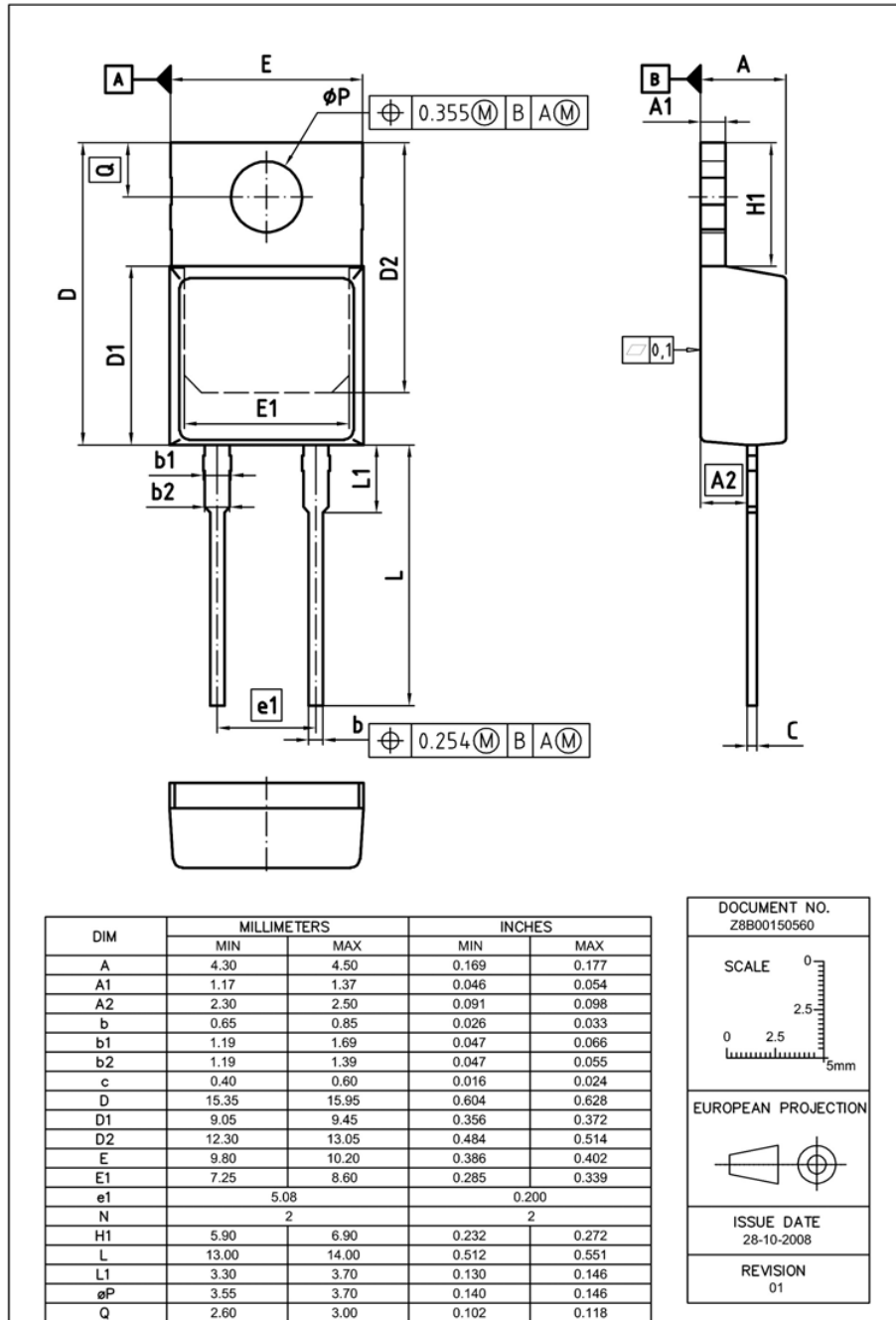
Figure 1 Outlines TO-220, dimensions in mm/inches
