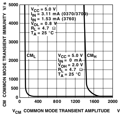
Figure 9. Common mode transient immunity vs. common mode transient amplitude.
