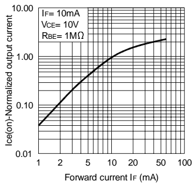
Fig.5 Output Current vs. Forward Current Curve
