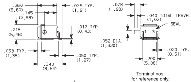
GP11MSABE SPST
