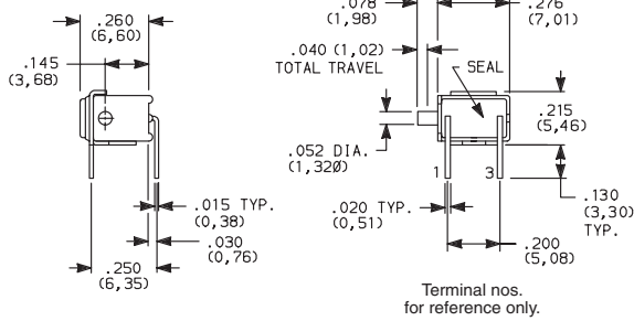
GP11MABE SPST
