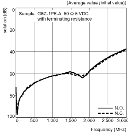
High-frequency Characteristics at 50 Ω (Isolation)
