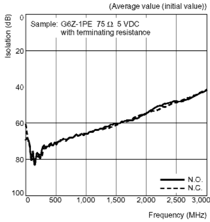
High-frequency Characteristics at 75 Ω (Isolation)
