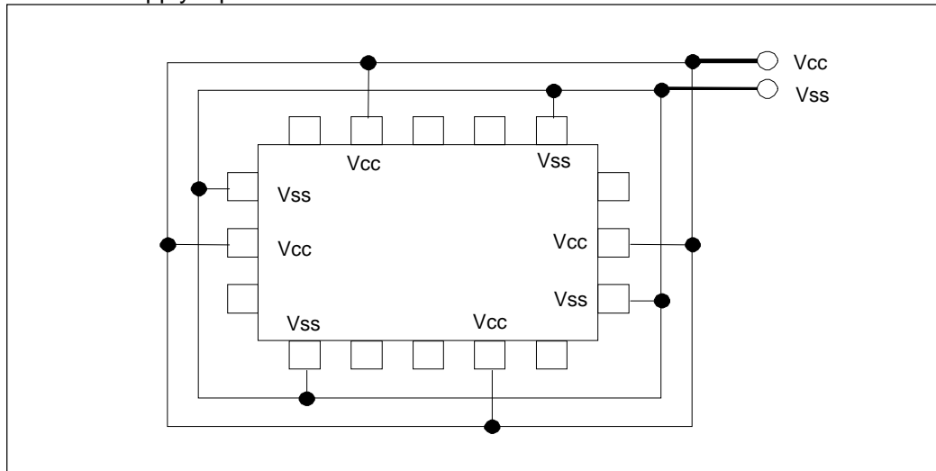
Figure 1 Power Supply Input Pins
