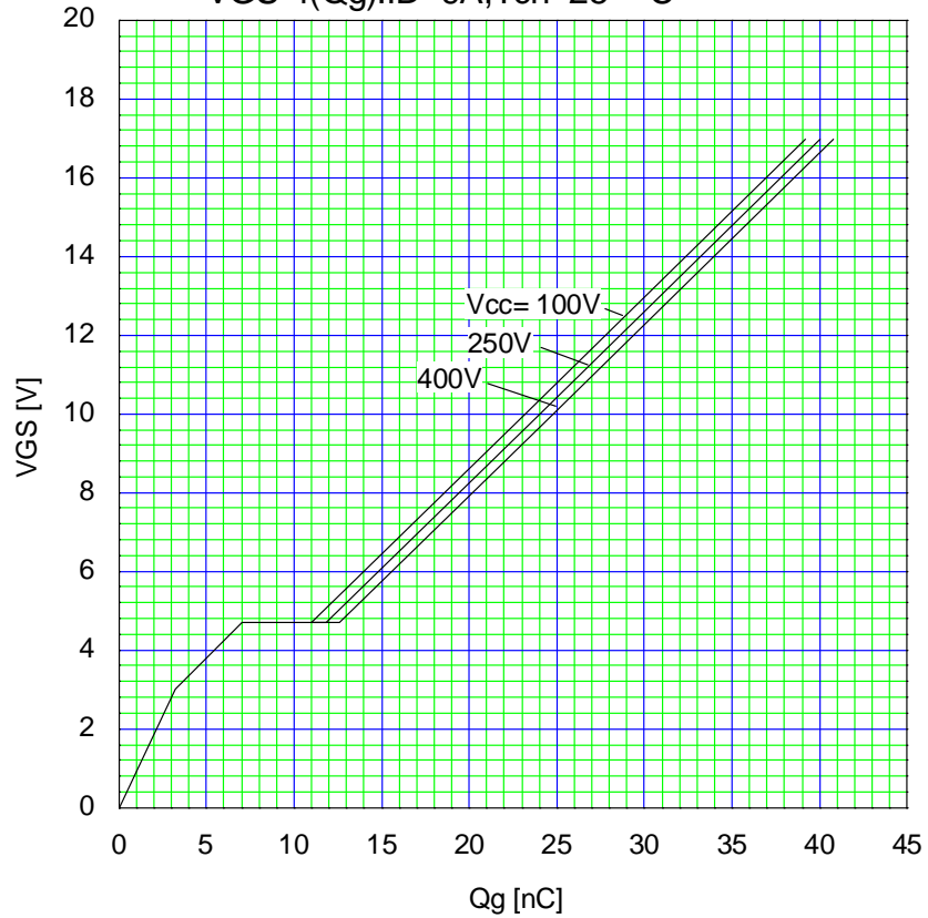
Typical Gate Charge Characteristics V_{GS}=f(Q_g):I_D=9A,T_{ch}=25\text{ }^\circ\text{C}
