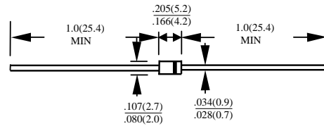
CASE : DO41 DIMENSIONS IN INCHES AND (MILLIMETERS)
