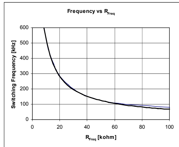
Figure 4. Switching Regulator Frequency vs. R_{Freq} Value.
