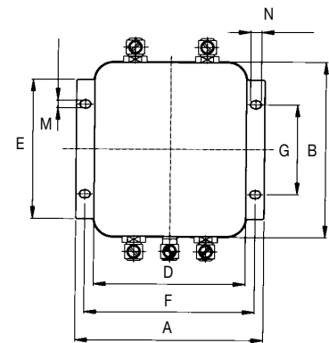
Housing L2
