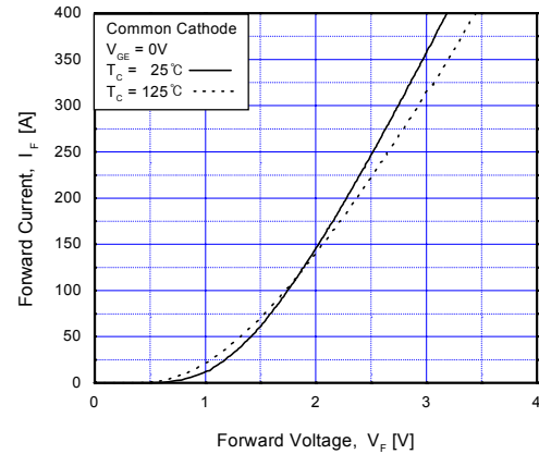
Fig 12. Forward Characteristics(diode)
