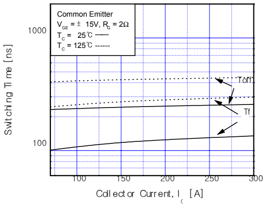
Fig 9. Turn-Off Characteristics vs. Collector Current
