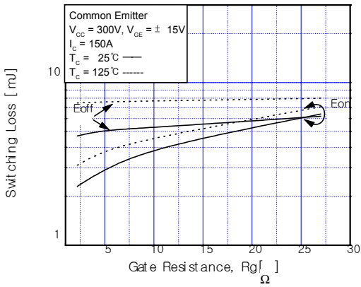
Fig 7. Switching Loss vs. Gate Resistance
