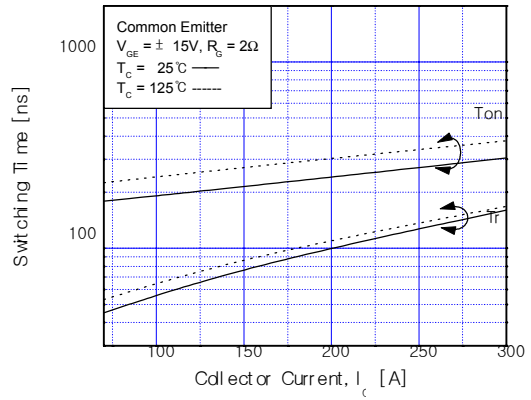
Fig 8. Turn-On Characteristics vs. Collector Current
