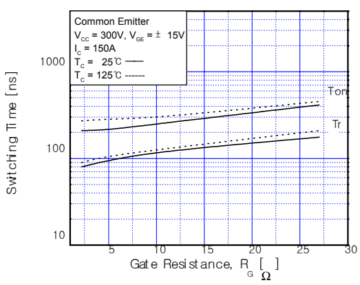
Fig 5. Turn-On Characteristics vs. Gate Resistance
