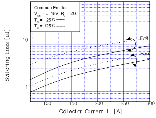
Fig 10. Switching Loss vs. Collector Current
