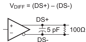
Figure 16. CTL Output Load and Transition Times
