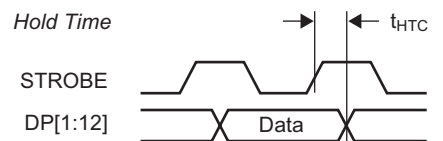
Figure 18. Serial Setup and Hold Time
