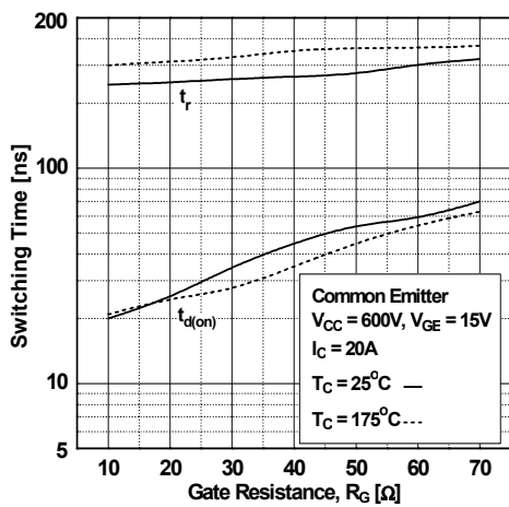
Figure 11. Turn-On Characteristics vs Gate Resistance
