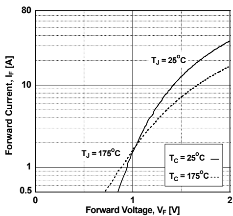
Figure 18. Forward Characteristics
