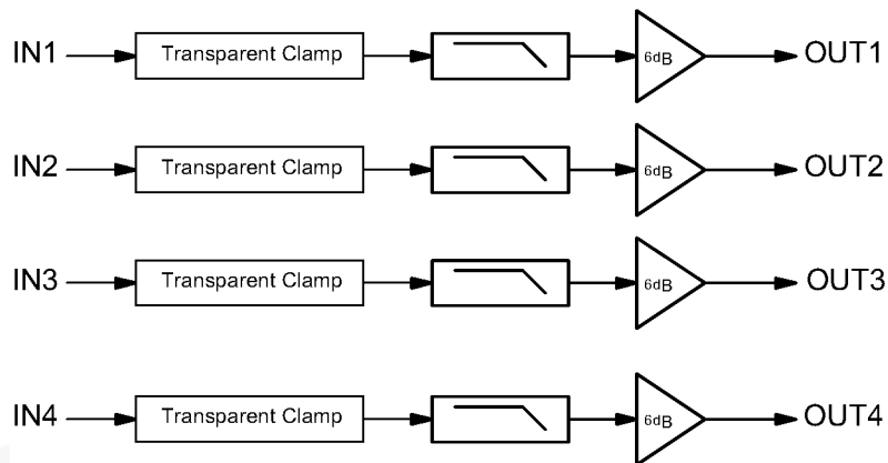
Figure 1. Block Diagram
