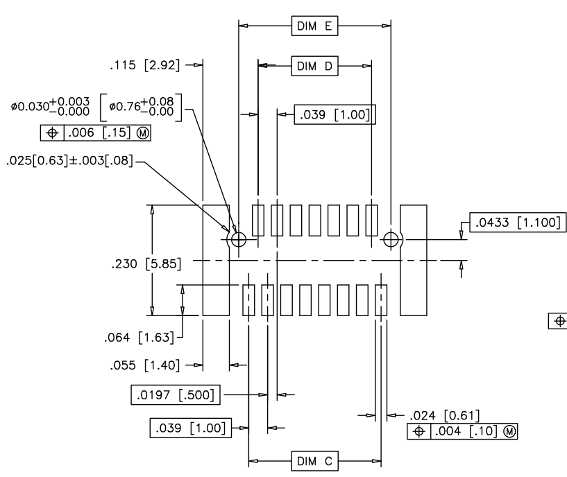
RECOMMENDED PAD LAYOUT FOR RECEPTACLE
