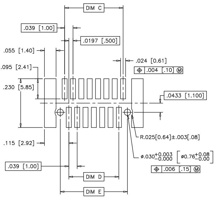
RECOMMENDED PAD LAYOUT FOR PLUG
