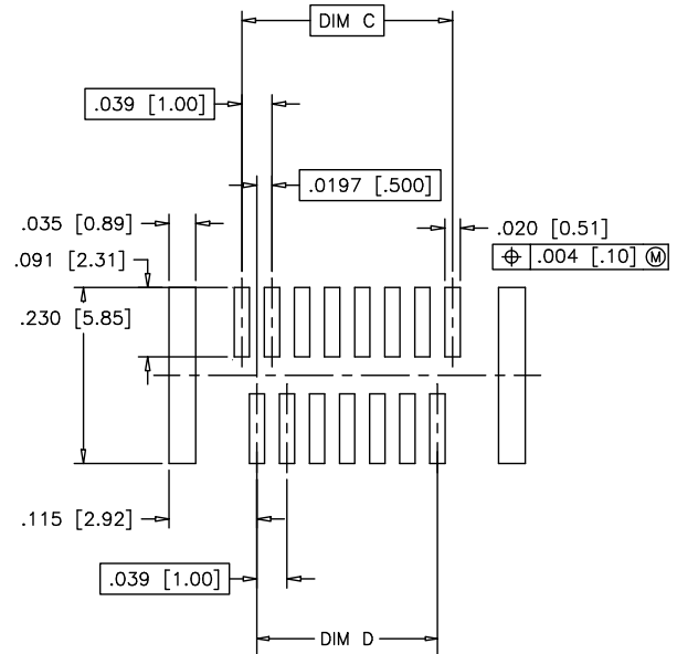
RECOMMENDED STENCIL LAYOUT FOR PLUG
