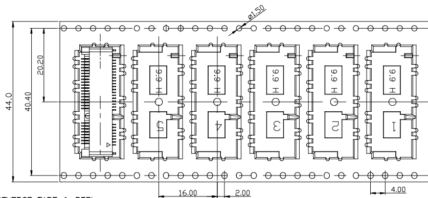
REVERSE TAPE & REEL (FOR -XX1LF)
