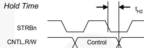
Figure 12. Master Read Setup and Hold Time
